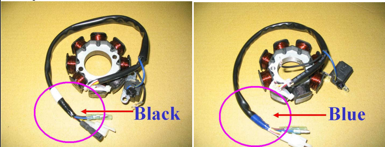
Picture 1 : original stator cable without blue tape Picture 2 : new stator cable with blue tape
